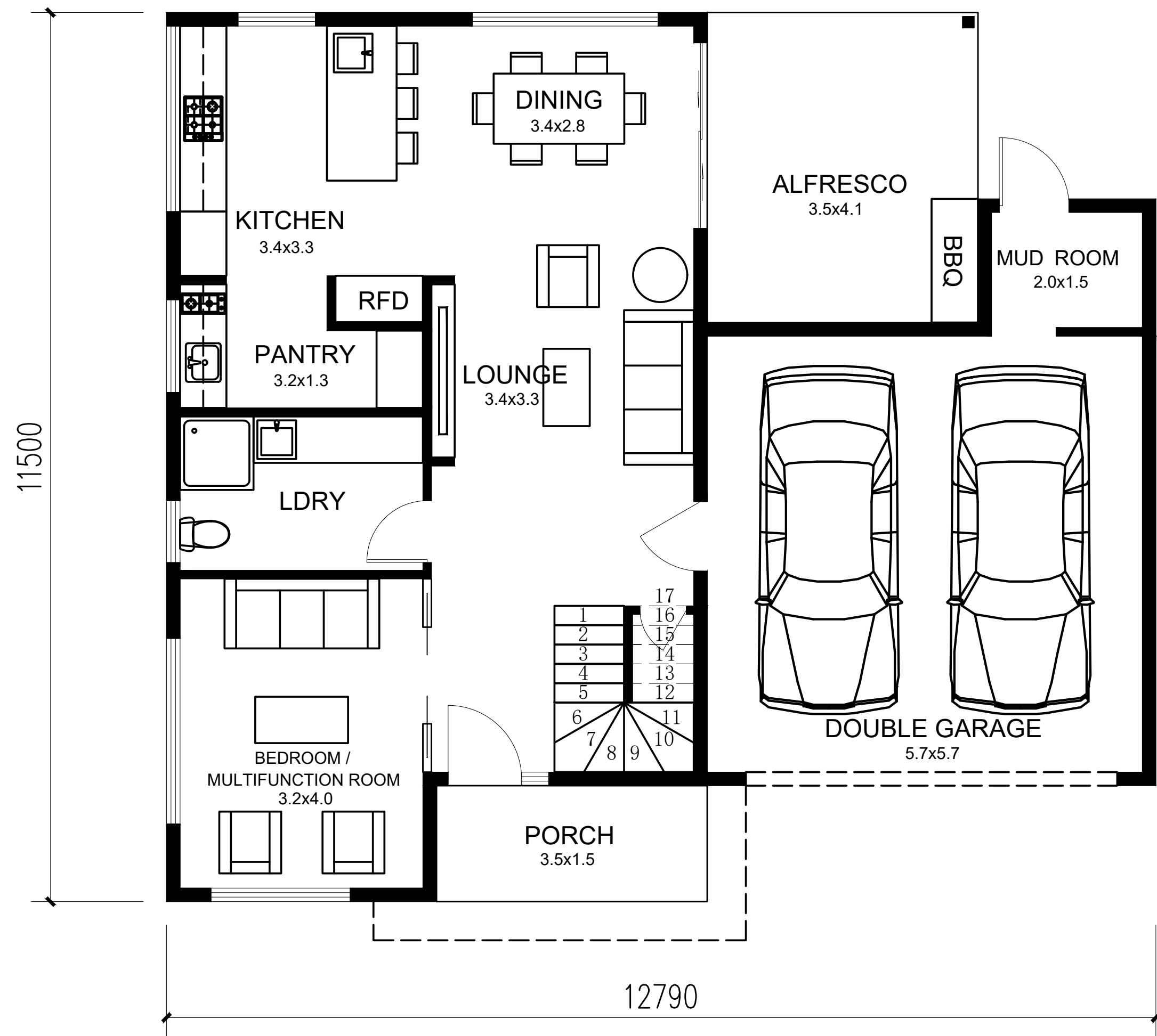
GROUND FLOOR
