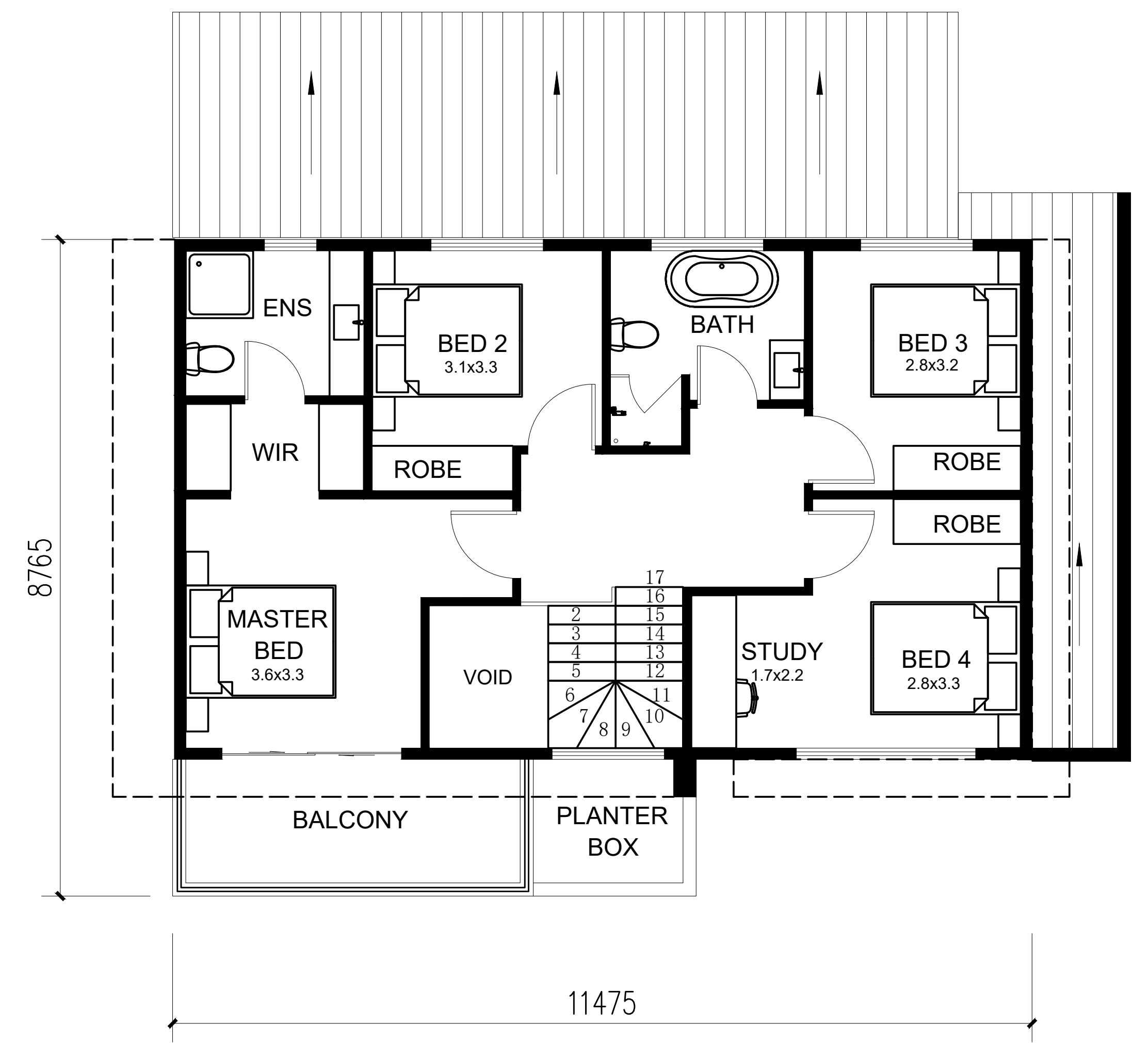
FIRST FLOOR
