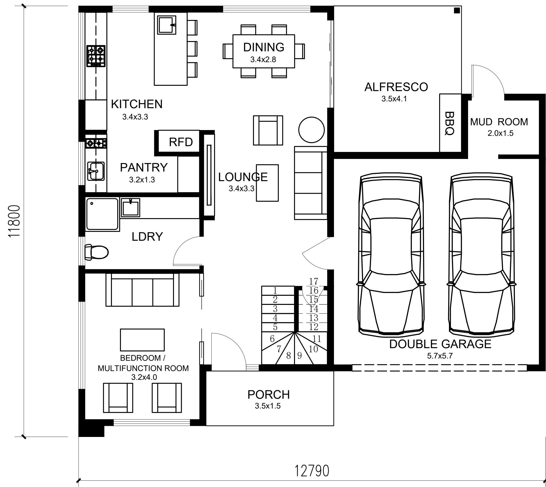
GROUND FLOOR
