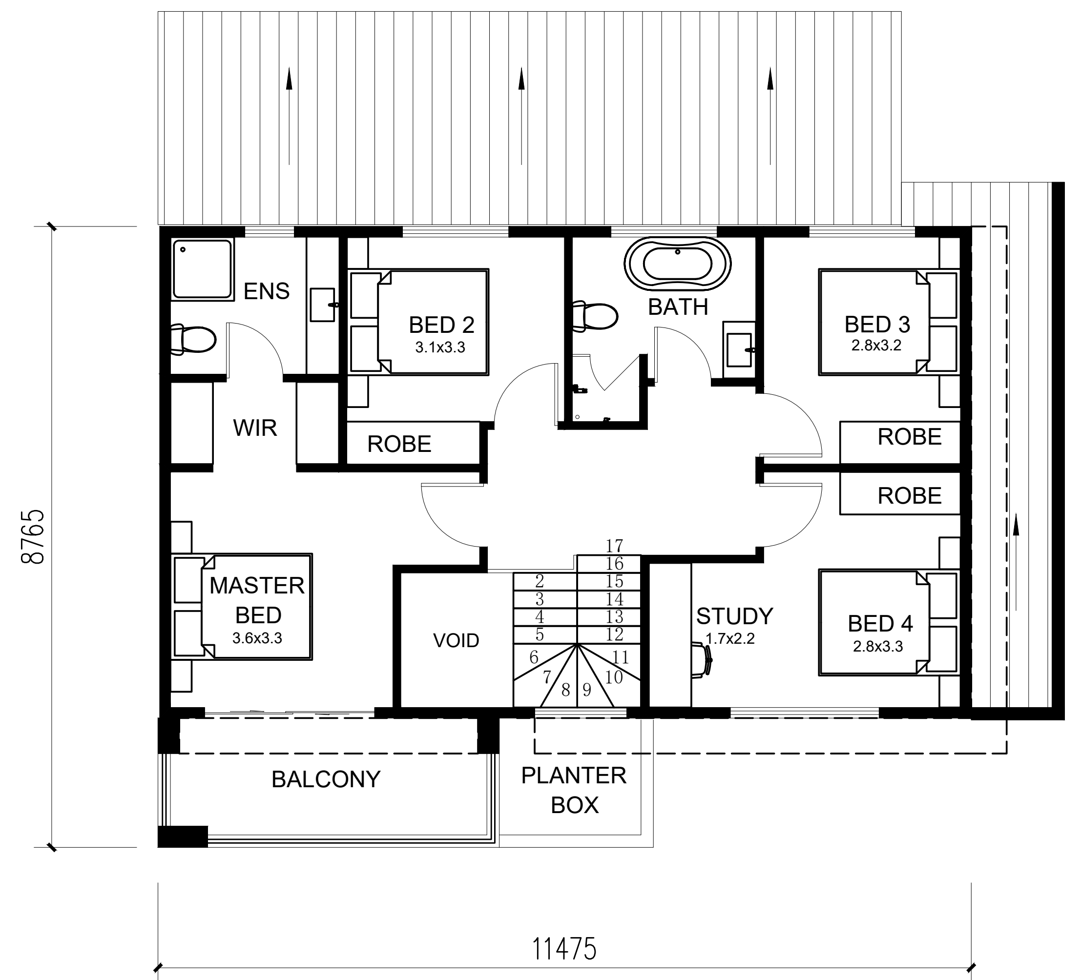
FIRST FLOOR
