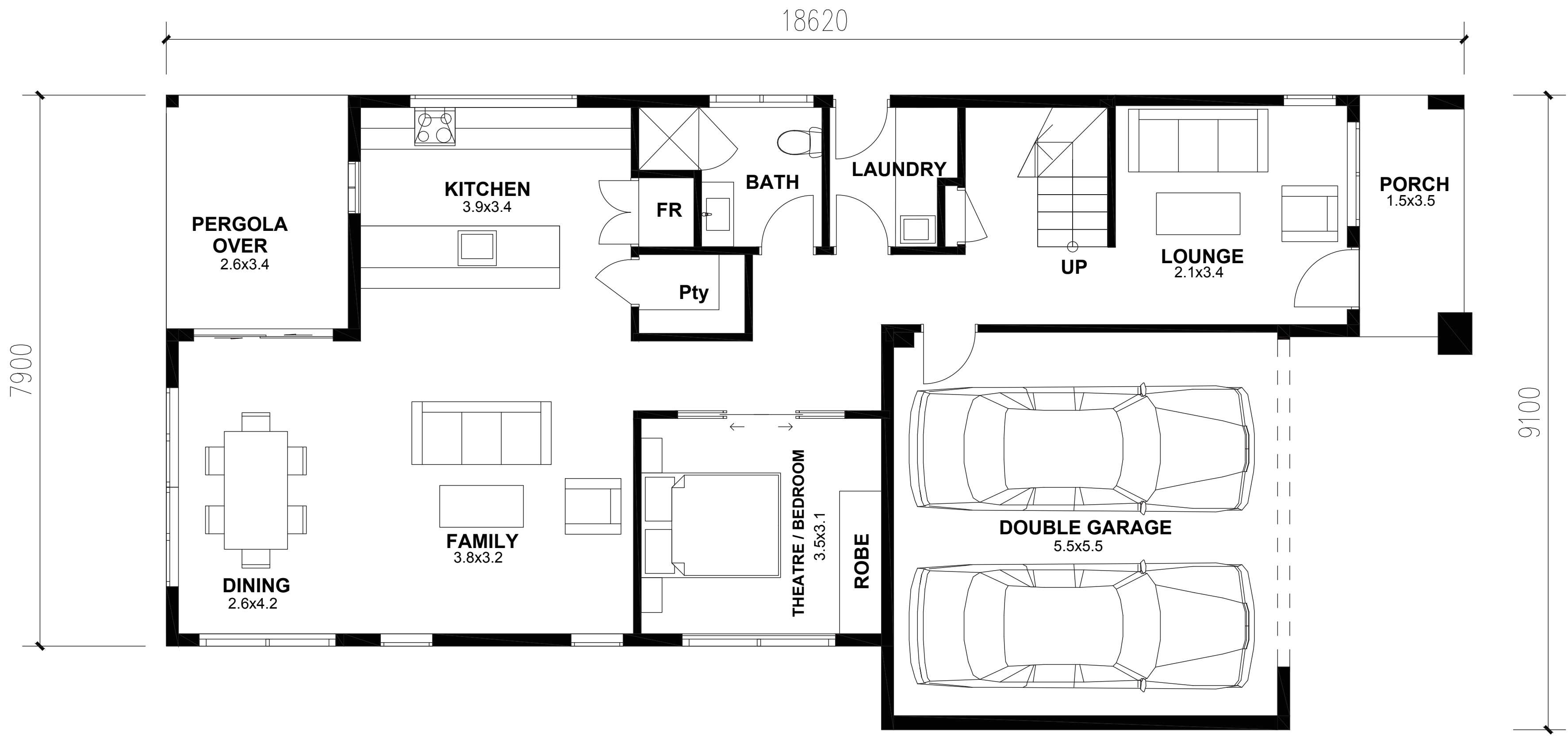
GROUND FLOOR
