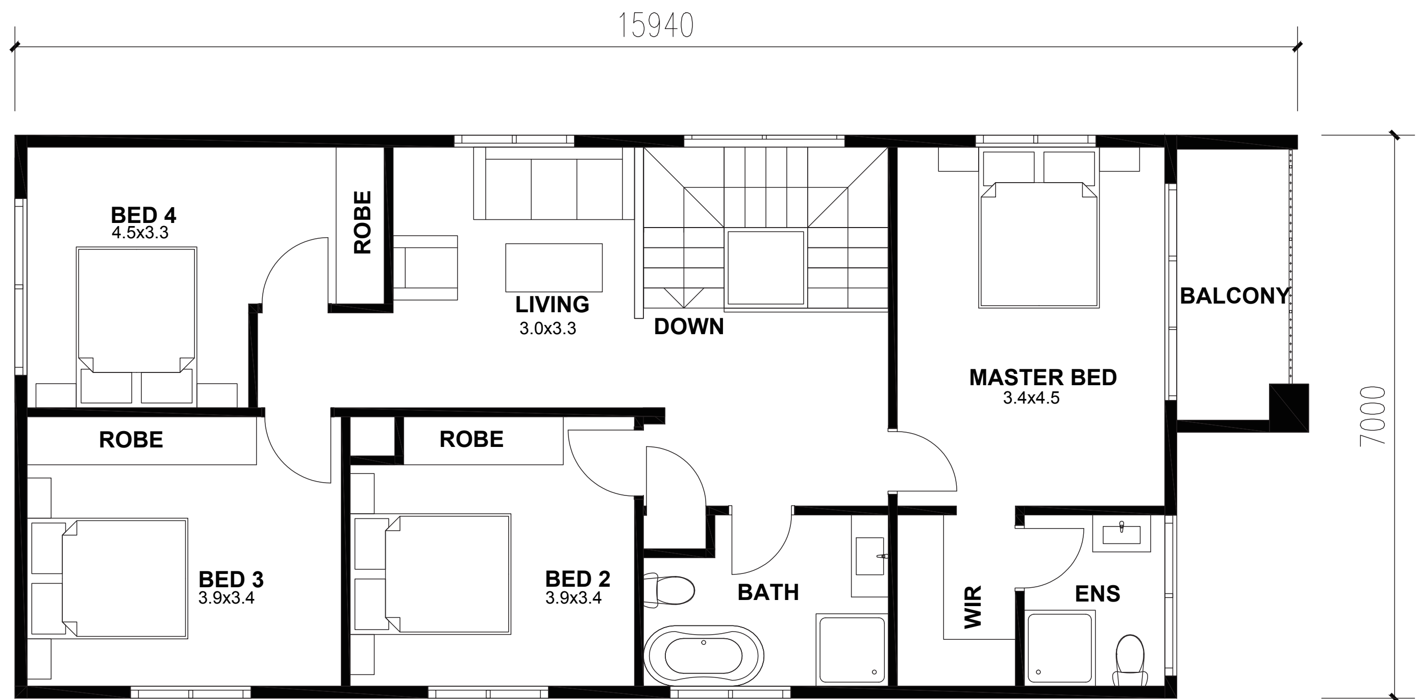
FIRST FLOOR
